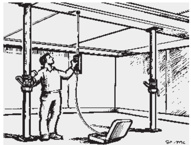
Using prods for checking ceiling shuttering level (One-handed spindle adjustment)
